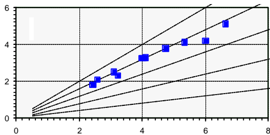
Fig. 15.3.17: Yf [kWh/kWp/d] vs. Yr [kWh/m²/d]
