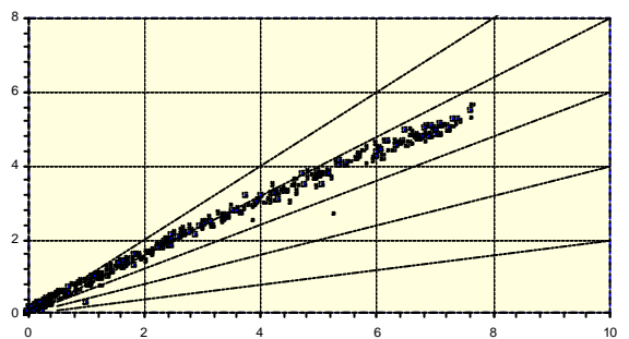
Fig. 4.3.5: Final Yield Yf vs. Reference Yield [kWh/kWp/d]
