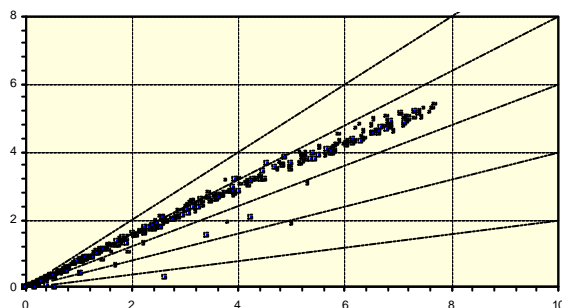
Fig. 6.3.5: Final Yield Y_f vs. Reference Yield Y_r [kWh/kWp/d]
