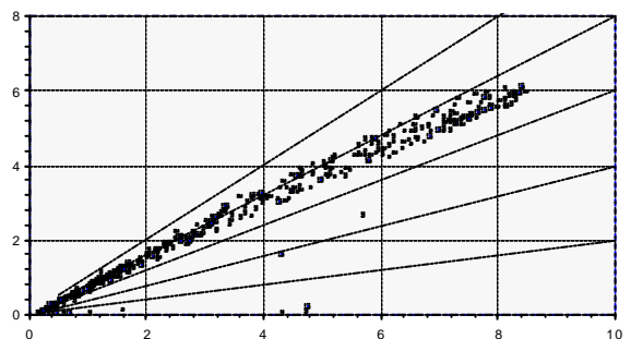
Fig. 10.3.5: Final Yield Y_f vs. Reference Yield [kWh/kWp/d]
