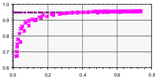
Fig. 15.3.5: \eta_{Inv} vs. P_{ac}/P_{nom} Inverter
