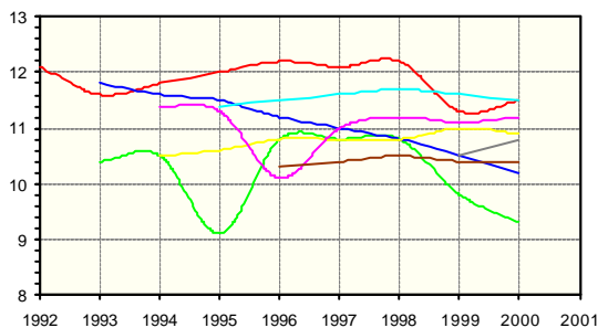
Fig 3.1.6: Generatorwirkungsgrad \eta_a^* : Arco Solar M55 (BAD) = rot, Solution/Siemens Solar 185 (FIN) = grün, Siemens Solar M55 (BRU) = dunkelblau, Siemens Solar M65 (STE) = gelb, Solution/Siemens 266 (DIS) = violett, Solution/Sharp 128 (WIN) = hellblau, GPV 110 (BUC) = braun, Siemens Solar SM110/24 (EWB) = grau
