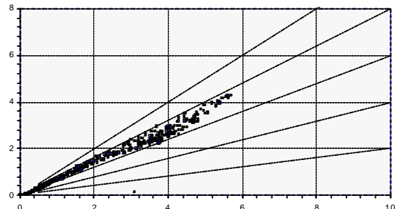
Fig. 9.3.5: Final Yield Yf vs. Reference Yield [kWh/kWp/d]
