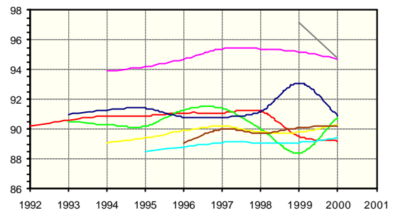
Fig 3.1.7: Wechselrichterwirkungsgrad \eta_i^* : Solcon 3 kW (BAD) = rot, Ecopower 15 kW (FIN) = grün, Ecopower 50 kW (BRU) = dunkelblau, Ecopower 15 kW (STE) = gelb, Ecopower 120 kW (DIS) = violett, Solarmax 50 kW (WIN) = hellblau, Schmidhauser P420 20 kW (BUC) = braun, Schmidhauser P430 30 kW (EWB) = grau
